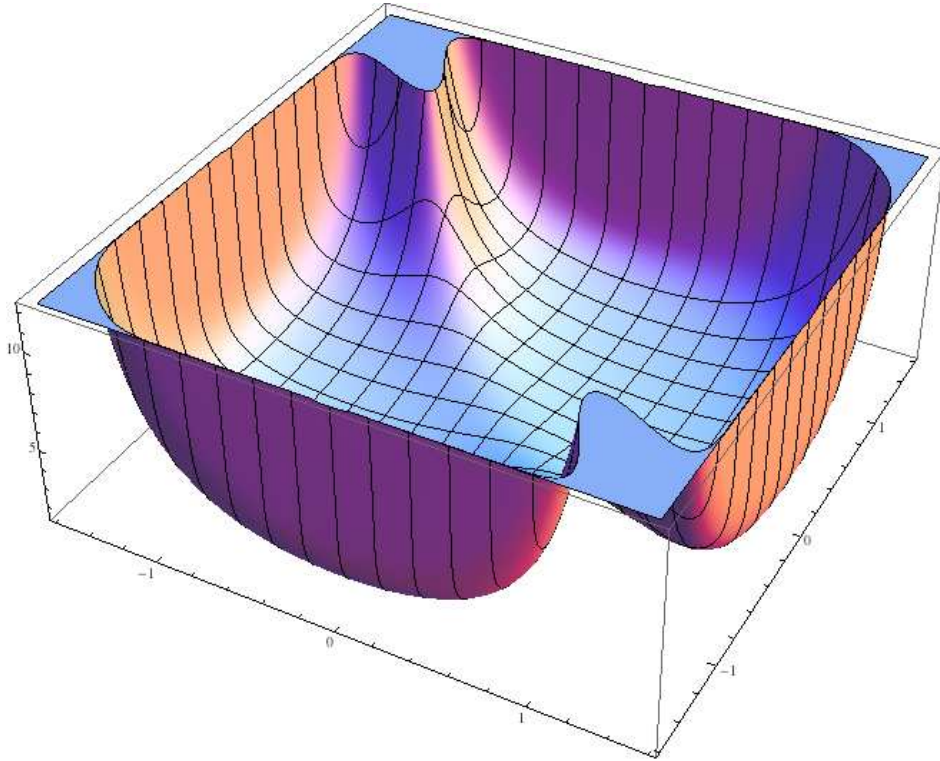
Figure 1: Plot of c_{5,0} integrand function in (233)
